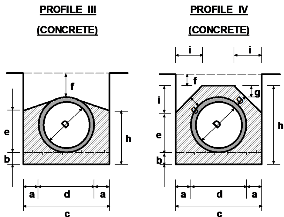
FIGURE C.14 - BEDDING AND HAUNCH PROFILES TYPES III & IV
