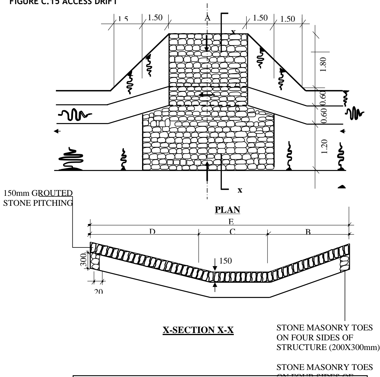
FIGURE C.15 ACCESS DRIFT
