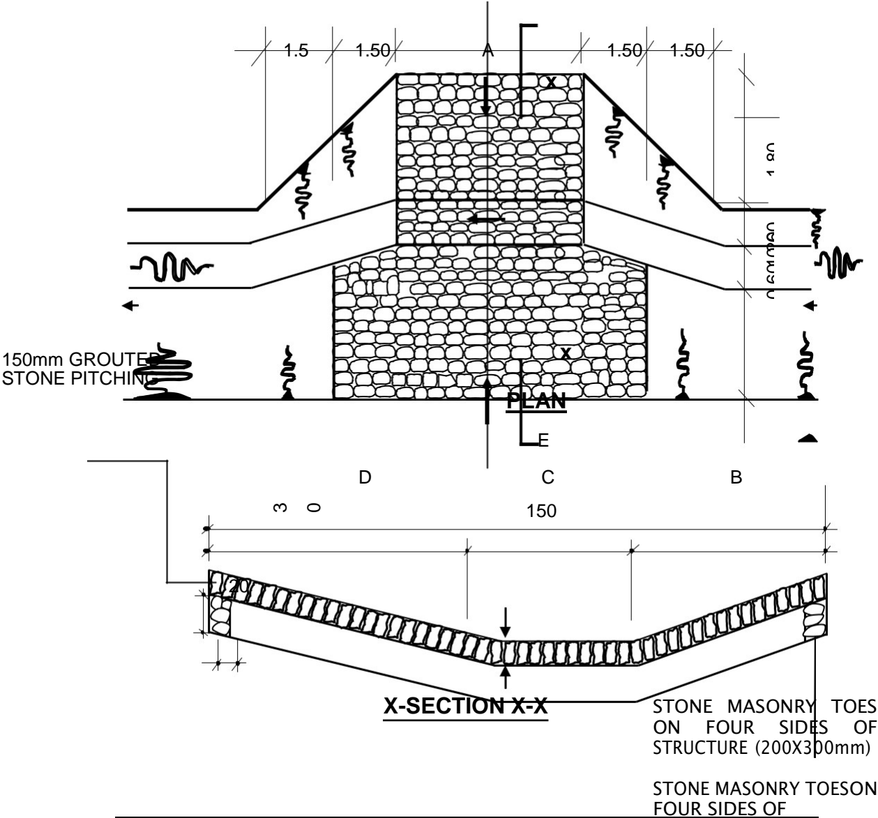
FIGURE C.15 ACCESS DRIFT
