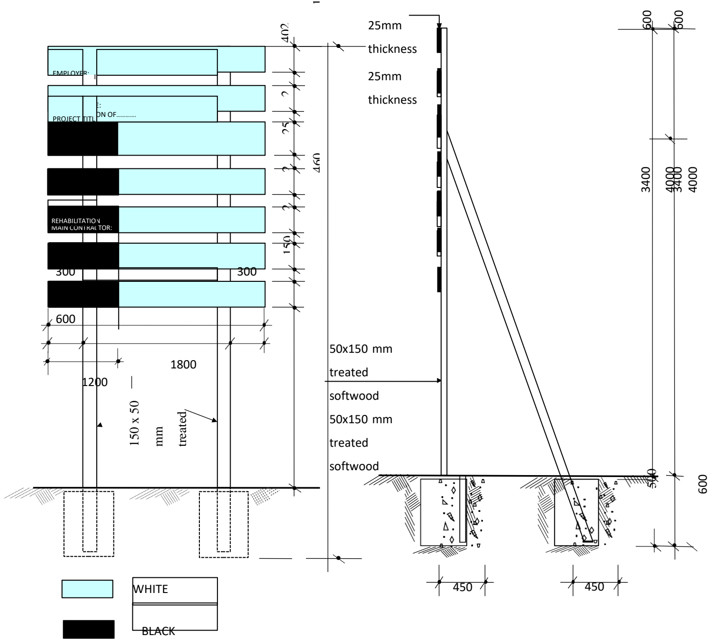
FIGURE C.17 - PUBLICITY SIGNBOARD
