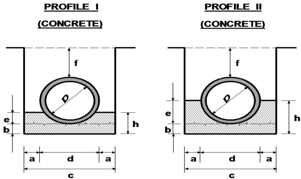
FIGURE C.13- BEDDING AND HAUNCH
