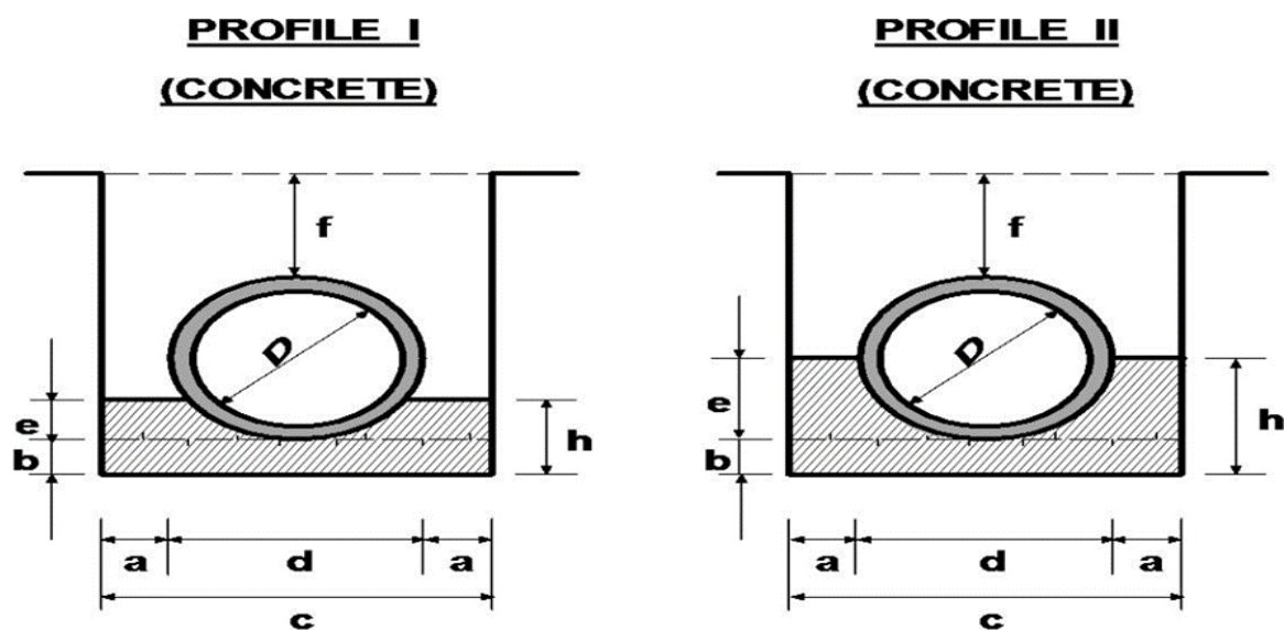
FIGURE C.13- BEDDING AND HAUNCH
