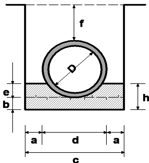
PROFILE I PROFILE II FIGURE C.13- BEDDING AND HAUNCH PROFILES TYPES I & II (CONCRETE) (CONCRETE)
