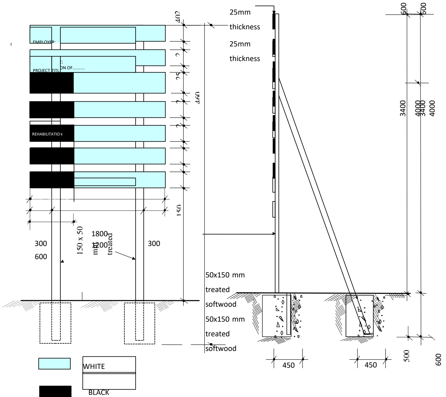
2 FIGURE C.17 - PUBLICITY SIGNBOARD
