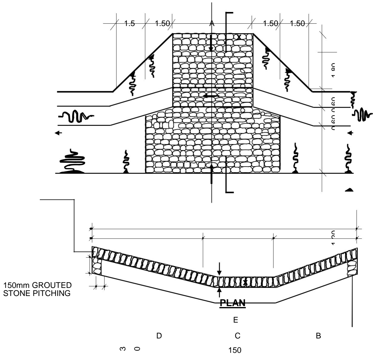
FIGURE C.15 ACCESS DRIFT
