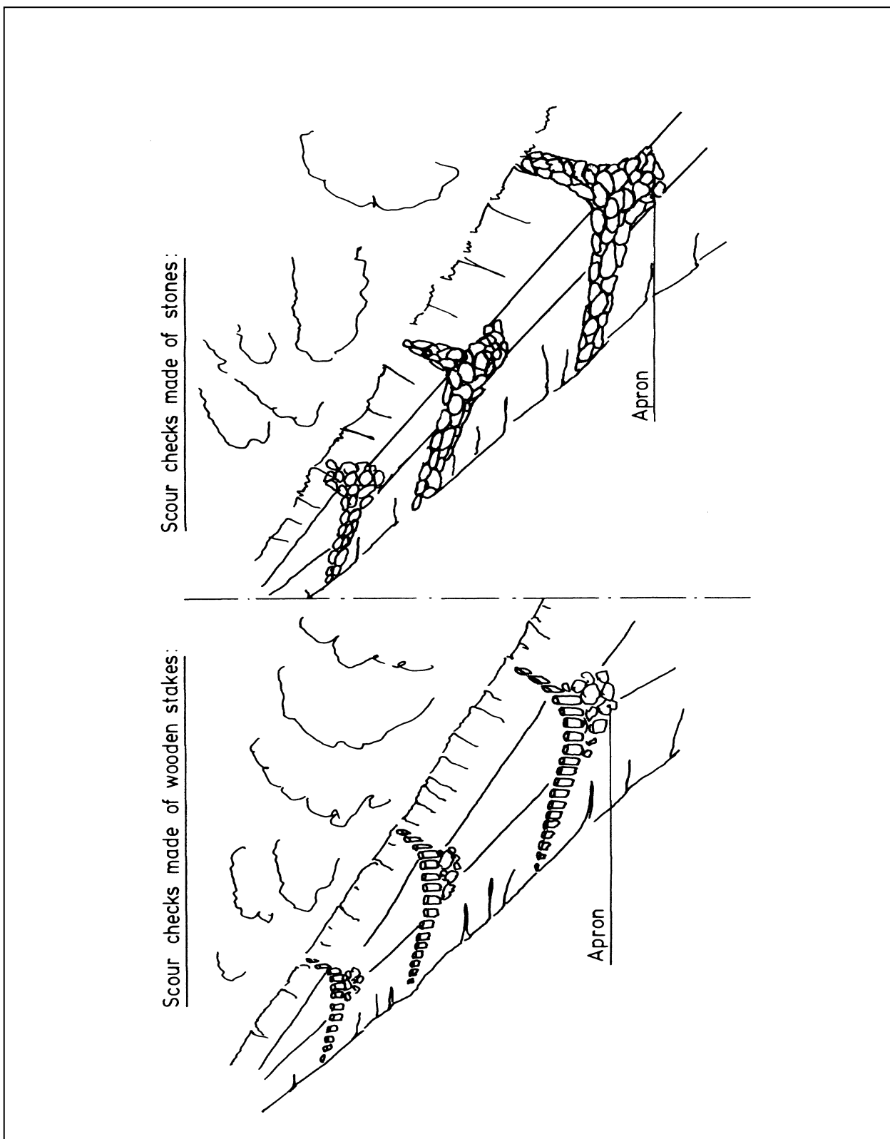
FIGURE C.4 - SCOUR CHECKS
