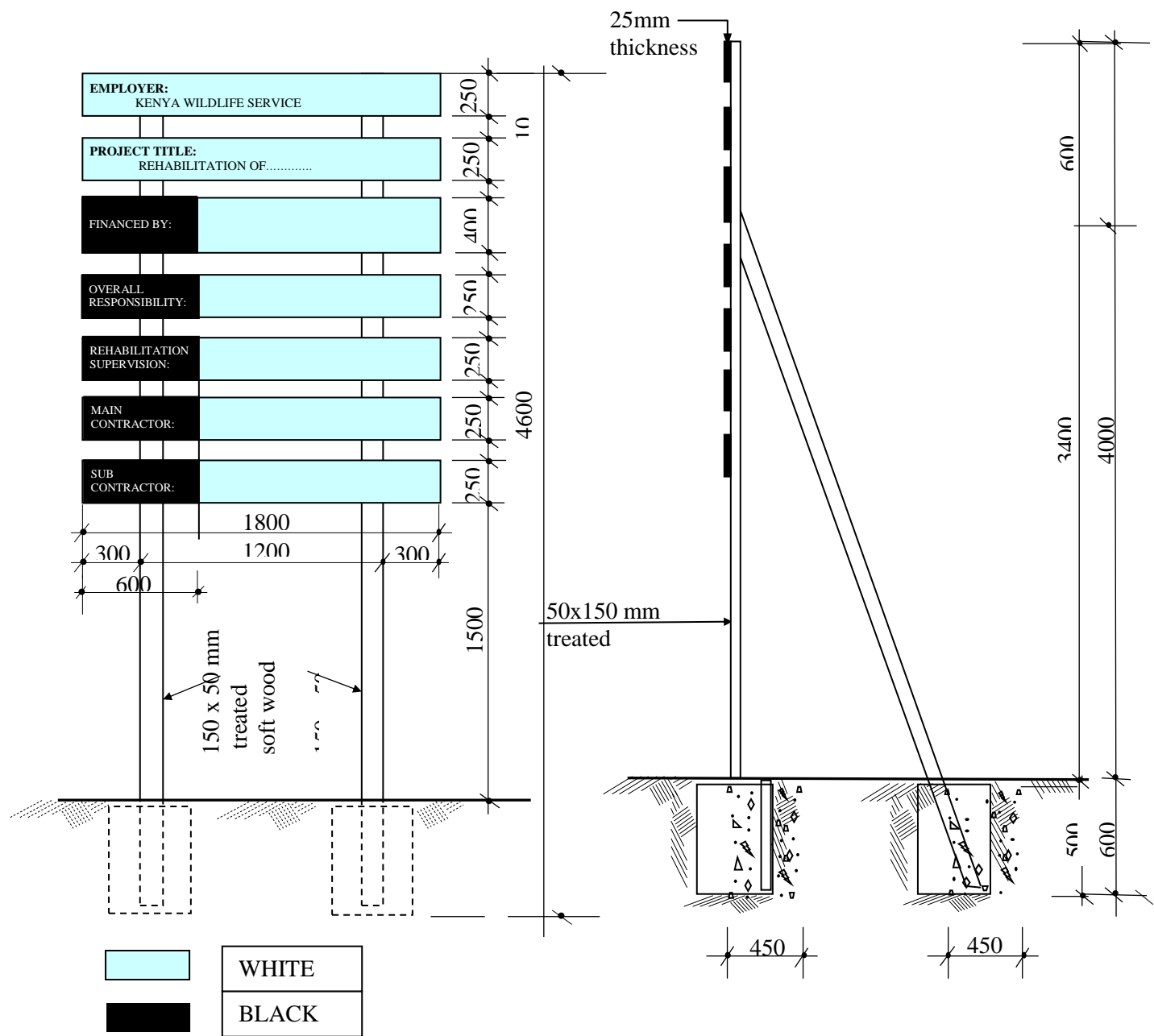
FIGURE C.17 - PUBLICITY SIGNBOARD
