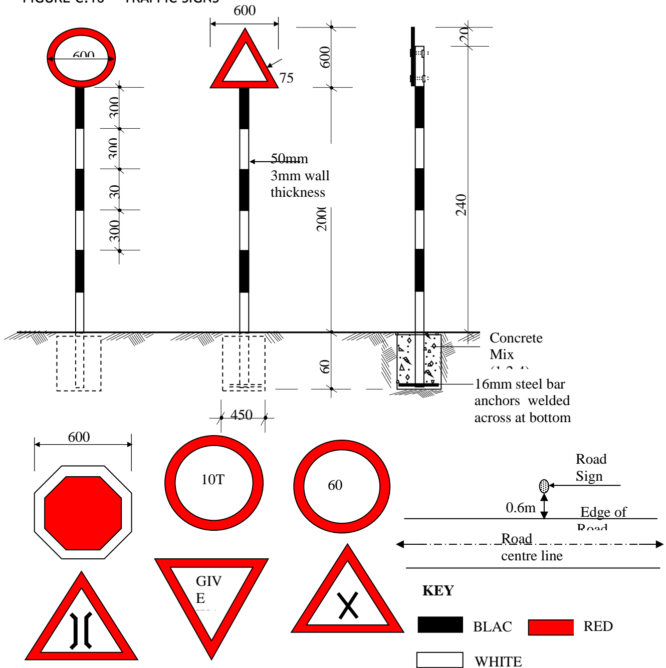
FIGURE C.16 - TRAFFIC SIGNS
