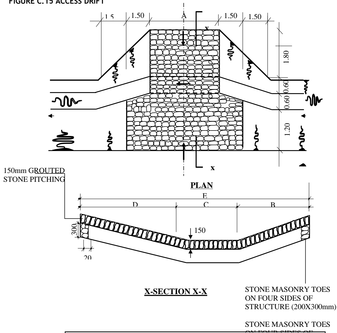
FIGURE C.15 ACCESS DRIFT
