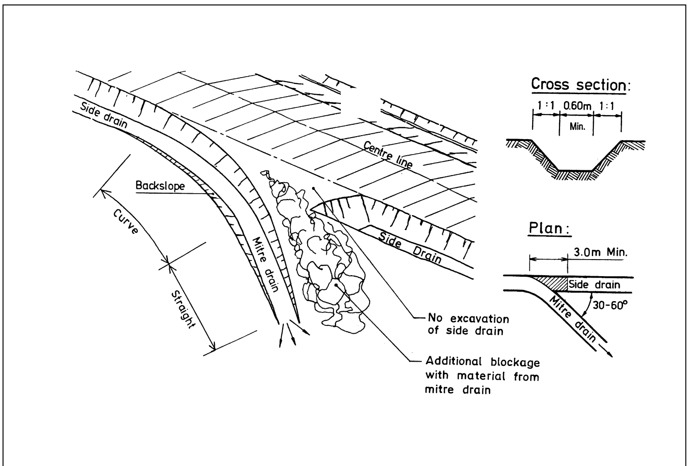
FIGURE C.4. – MITRE DRAINS
