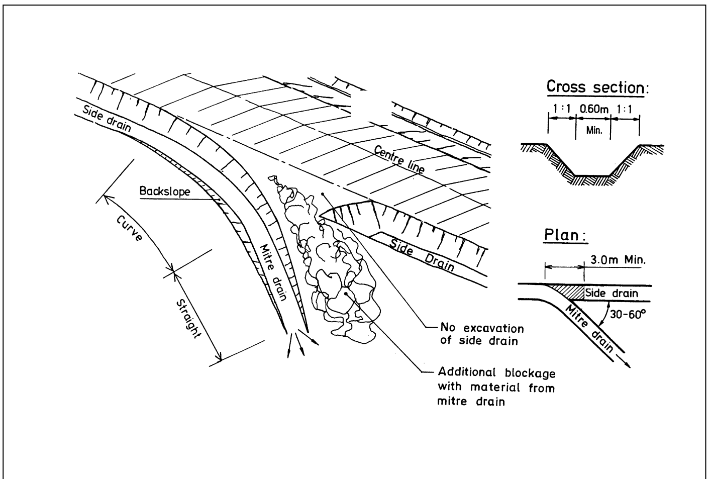
FIGURE C.4. – MITRE DRAINS
