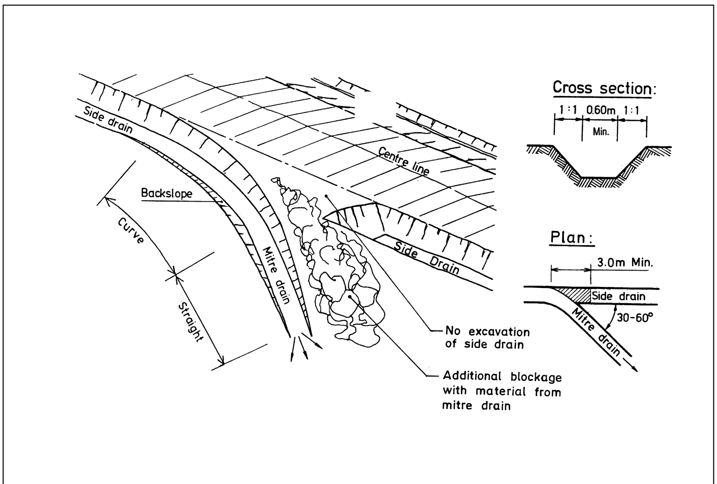
FIGURE C.4. – MITRE DRAINS
