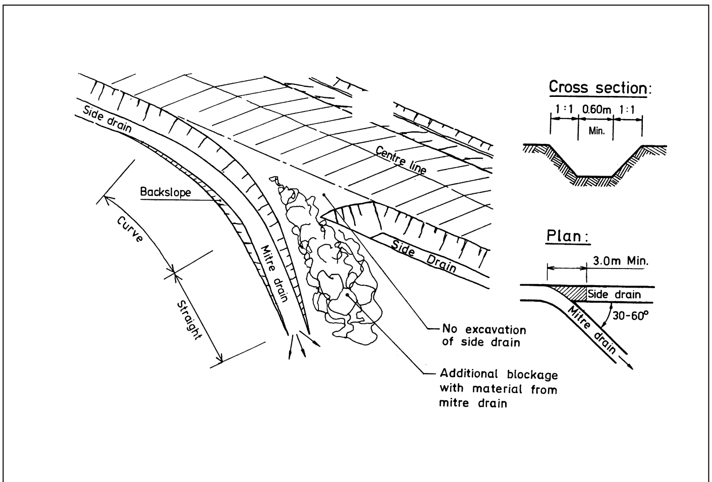
FIGURE C.4. – MITRE DRAINS
